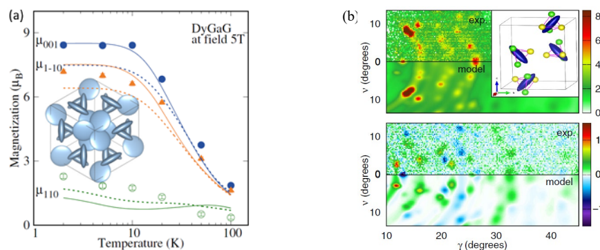
Fig.1: (a) Magnetization components versus temperature for DyGaG. Insets show magnetization ellipsoids. (b) The measured and calculated flipping sum (top) and difference (bottom) diffraction patterns collected on Co([CH 3 ) 2 N] 2 CS) 2 Cl 2 at 2K, 5T.
