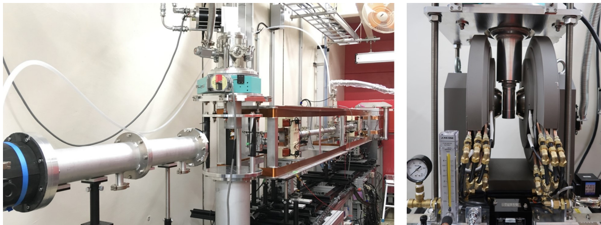
Figure: (left) MIEZE spectrometer at BL06. (right) Newly installed magnet and cold head.
