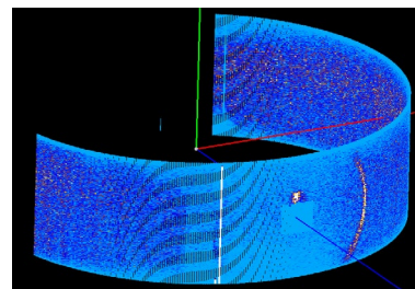
NEAT Detector map showing complete detector coverage of 240° by 40° from the ^3\text{He} cell.
