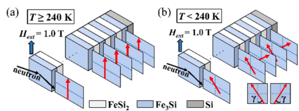
Fig 1. (a) Schematic figure of collinear ferromagnetic structure of \text{Fe}_3\text{Si}/\text{FeSi}_2 superlattice, and (b) one of non-collinear ferromagnetic structure with transverse anti-ferromagnetic order.
