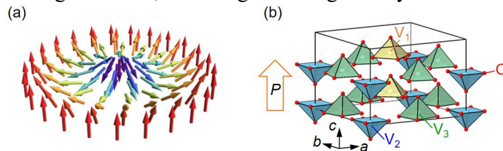
Figure 1 (a) Neel-type skyrmion. (b) Crystal structure of \text{VOSe}_2\text{O}_5 .
